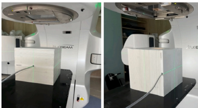
Figure 1. Slab phantom setup for CBCT dosimetry measurements using a Farmer-type ionisation chamber. Left: central position; right: peripheral position.
